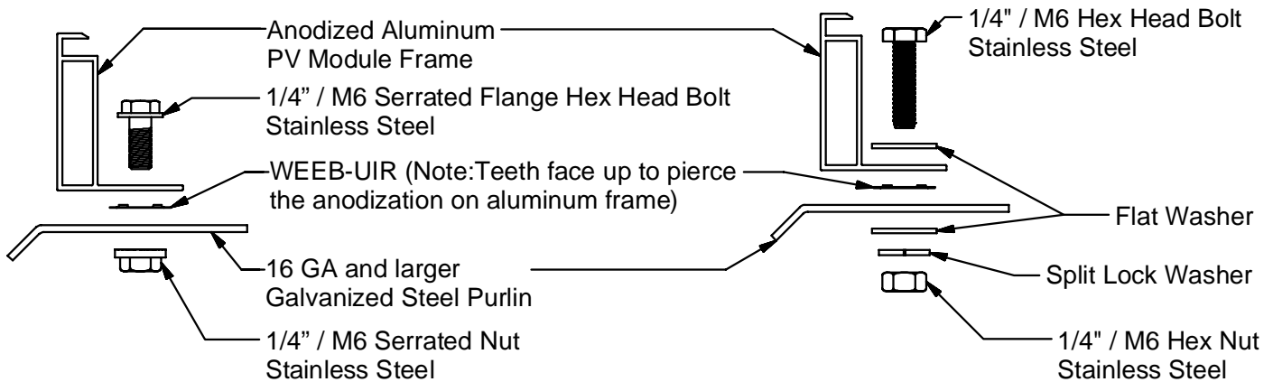
Fig 2: Bottom Mounting-With Washers
